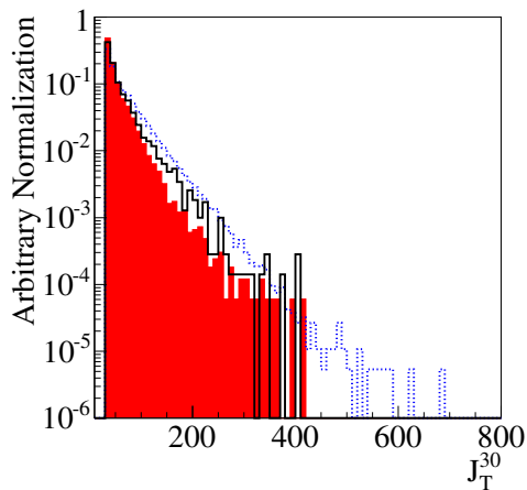
FIG. 21: The J_T^{30} distribution without the N_{\text{jet}}^{30} \geq 3 requirement in the Z +jet data (black line), compared to “X”+jet data selected with the jet triggers (red histogram) and to “X”+jet data selected with the electron triggers (dotted blue line).
