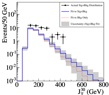
FIG. 29: Prediction for the J_T^{30} distribution in standard model Z \rightarrow \mu\mu events, with and without the presence of a 200 \text{ GeV}/c^2 b' signal introduced. The difference between the two predictions is small compared to the excess of signal at large J_T^{30} .
