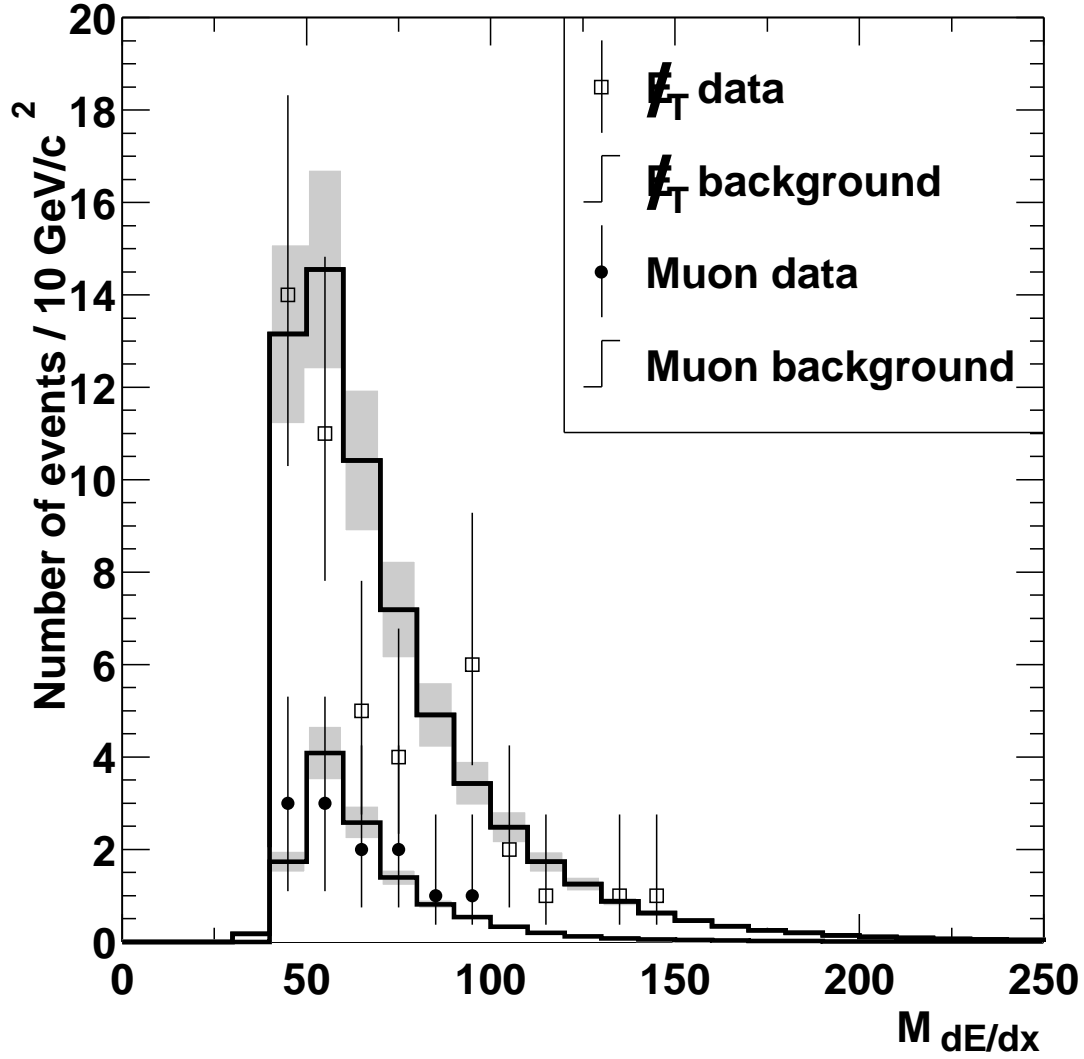
Figure 2: Observed M_{dE/dx} distribution for tracks passing all the cuts for the strong production search in the muon trigger and \cancel{E}_T trigger data samples [10]. The curves are the expected background distributions which have an uncertainty of about 15% which is shown by the gray bands.
