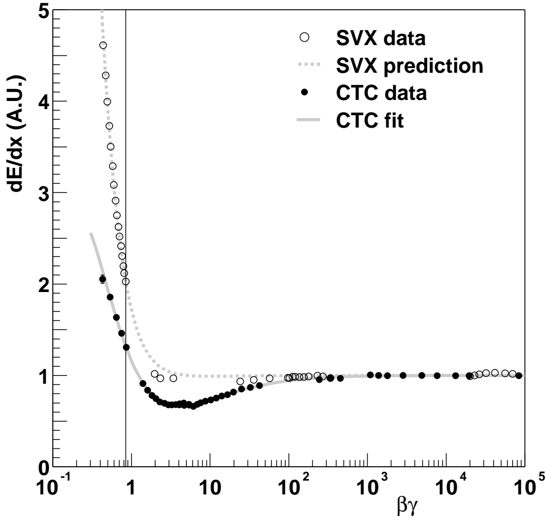
Figure 1: dE/dx measurements in control samples are compared to predictions for SVX' (open points) and CTC (solid points). The CTC prediction is a fit including detector effects. The SVX' prediction is the Bethe-Bloch formula. The agreement is good in the low and high \beta\gamma regions important to this search.
