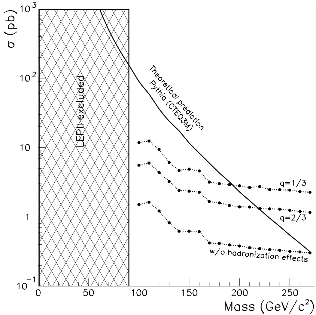
Figure 3: Limits set at 95% confidence level on the production cross section of long-lived fourth generation quarks are compared to the theoretical prediction.
